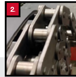
2. 4" double pitch roller chain has 70,000 lbs. pull strength per side for a total 140,000 lbs. pull strength.
